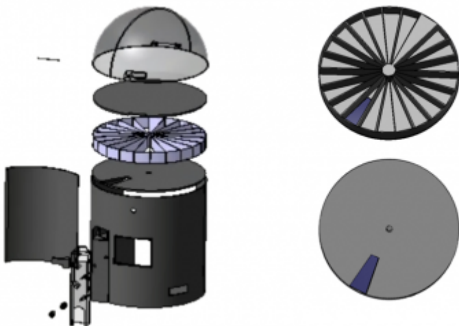
Figure 47: Billy's structure and mechanism
